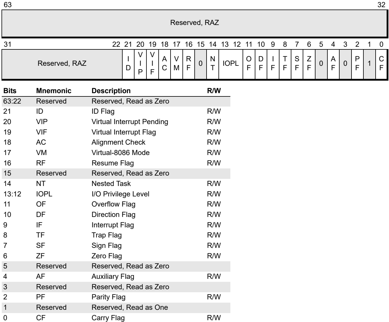
Figure 3-7. RFLAGS Register
