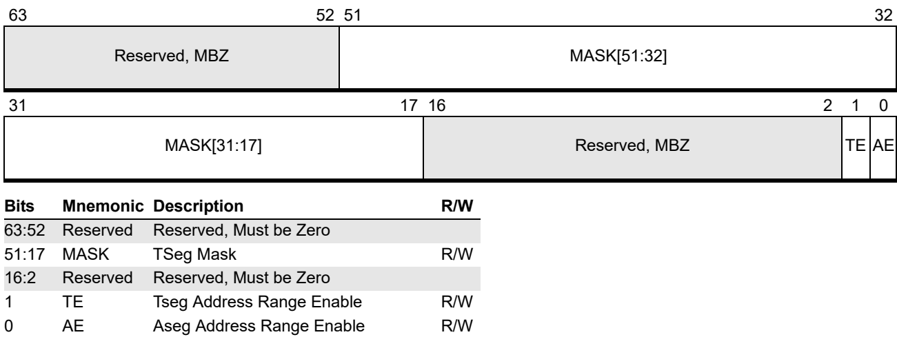
Figure 10-5. SMM_MASK Register Format
